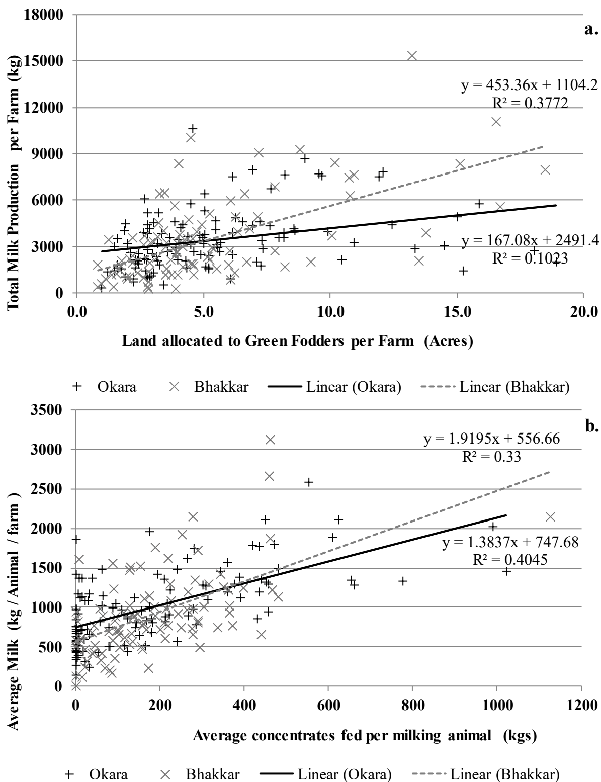
Figure 2. Linear regressions for (a) total milk production per farm and land allocation for green fodders, and (b) average milk production per milking animal per farm for the concentrates fed in irrigated Okara and arid Bhakkar districts of Punjab
