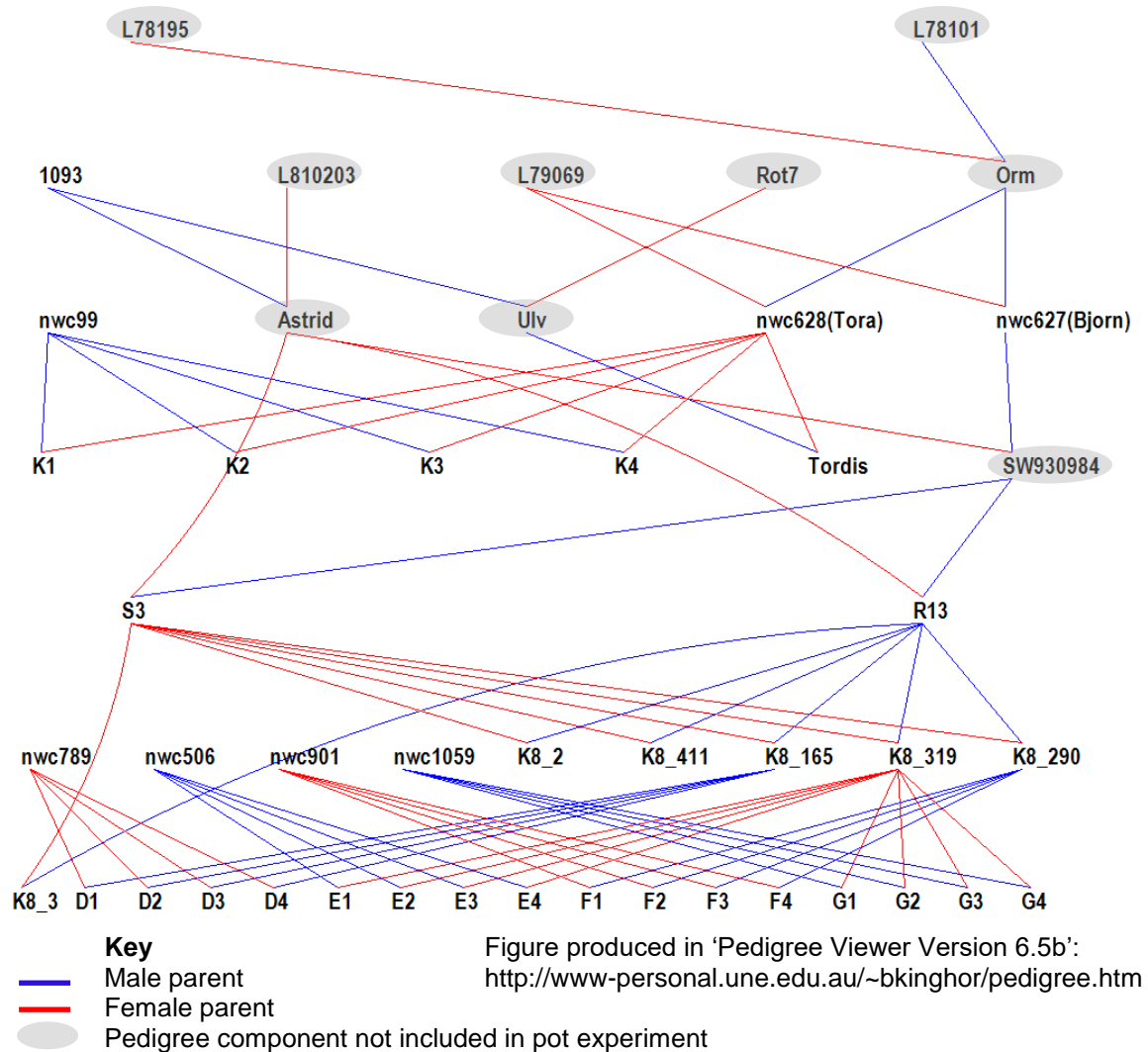
Figure 2.1 Pedigree plot.
