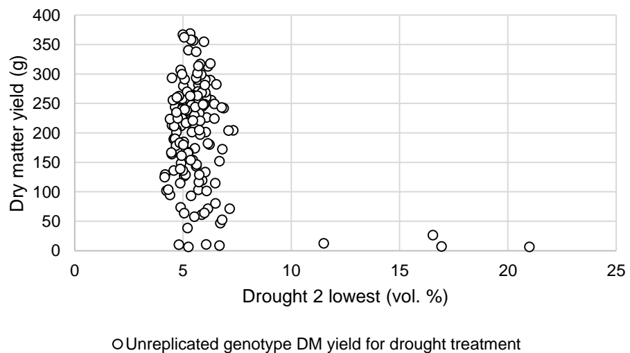
Figure 2.27 Final yield of droughted plants and lowest growth media moisture content during D2.
