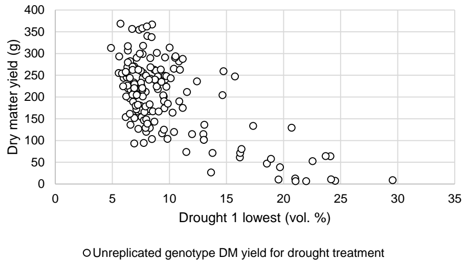
Figure 2.26 Final yield of droughted plants and lowest growth media moisture content during D1.
