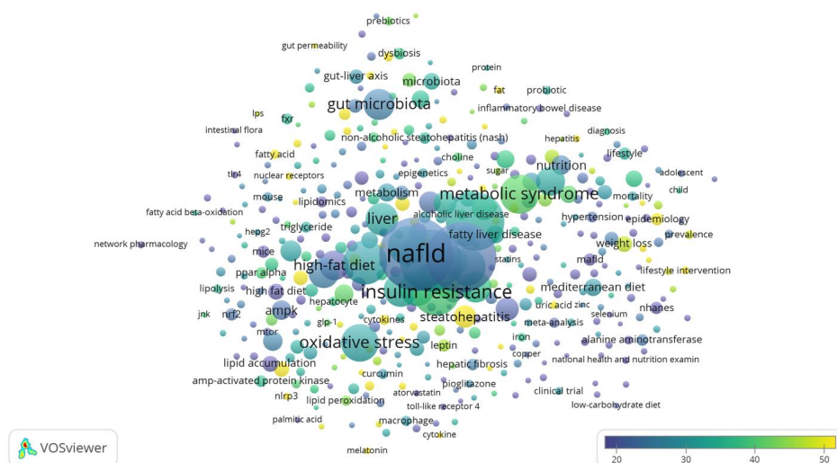
Fig. 3. Term map of recurring author keywords of the papers. The node color represents the citations per paper (CPP) of the terms, whereas the node size represents the number of papers, and the inter-node distance represents how frequently the terms co-occurred with each other in the same papers.
