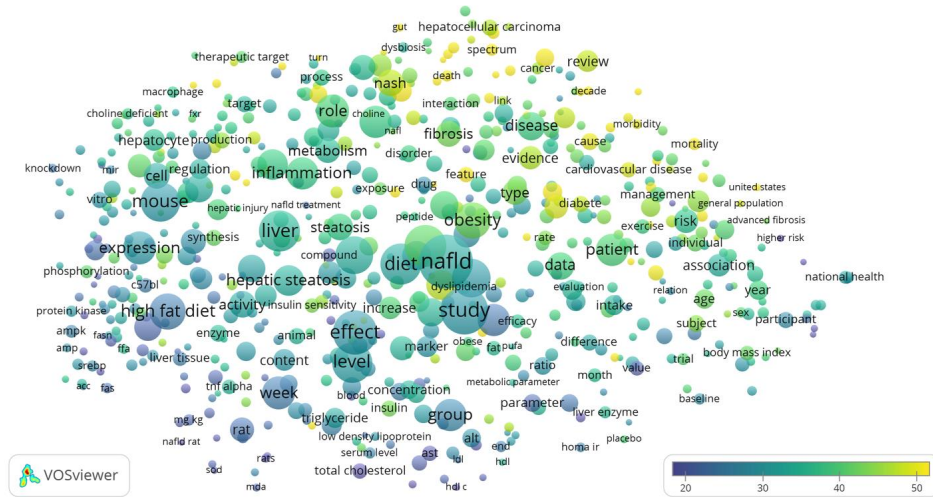
Fig. 2. Term map of recurring terms in the titles and abstracts of the papers. The node color represents the citations per paper (CPP) of the terms, whereas the node size represents the number of papers, and the inter-node distance represents how frequently the terms co-occurred with each other in the same papers.
