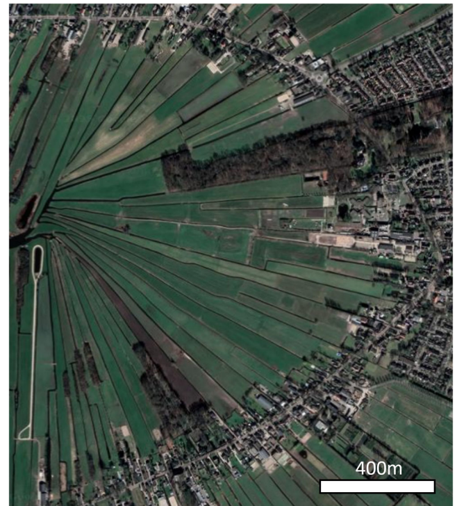
Fig. 2 | Drainage ditches can give clues to lost landscapes. Ditches in the Netherlands (52.20°N 5.12°E) show a wedge-shaped structure, and point towards the top of the (now missing) dome of a destroyed raised bog. Maps data: Google Earth, Maxar Technologies.
