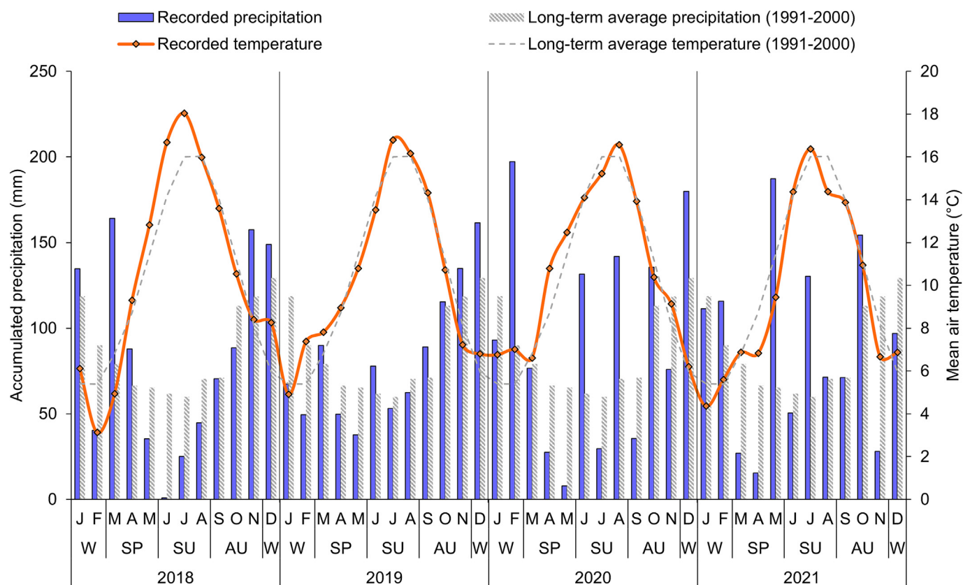
Fig. 3. Monthly recorded (2018–2021) and long-term (1991–2000) average temperatures and accumulated precipitation recorded at the met station near the dairy x beef cattle grazing study. *Recorded data (2018–2021) obtained from North Wyke Farm Platform data portal ( https://nwfp.rothamsted.ac.uk ); Long-term average data (1991–2000) obtained from Met Office (2025). W, winter; SP, spring; SU, summer; AU, autumn. Letters J to D within each year in the x-axis represent the months (January to December, respectively).
